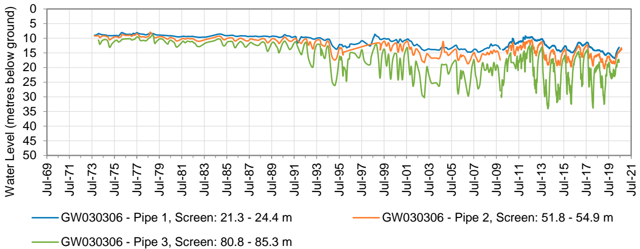
Figure 12: Hydrograph of monitoring bore GW030306
