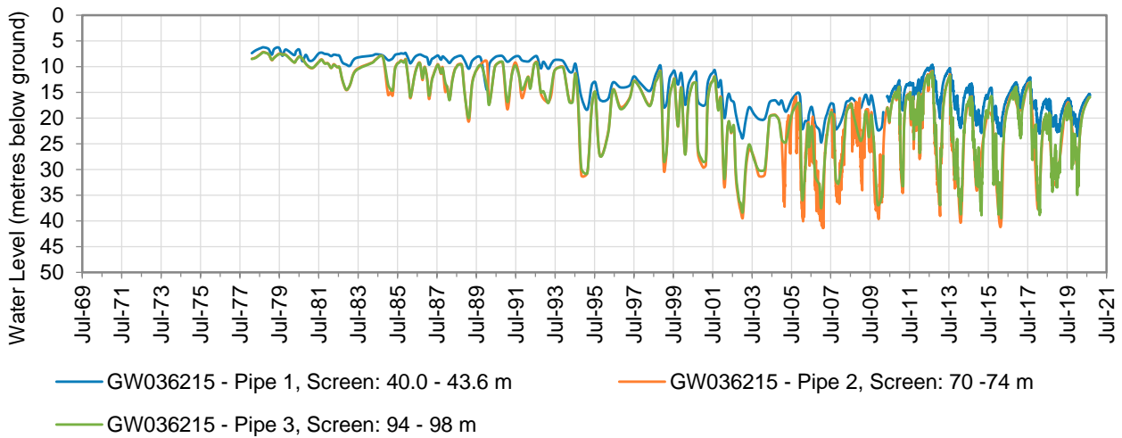
Figure 11: Hydrograph of monitoring bore GW036215
